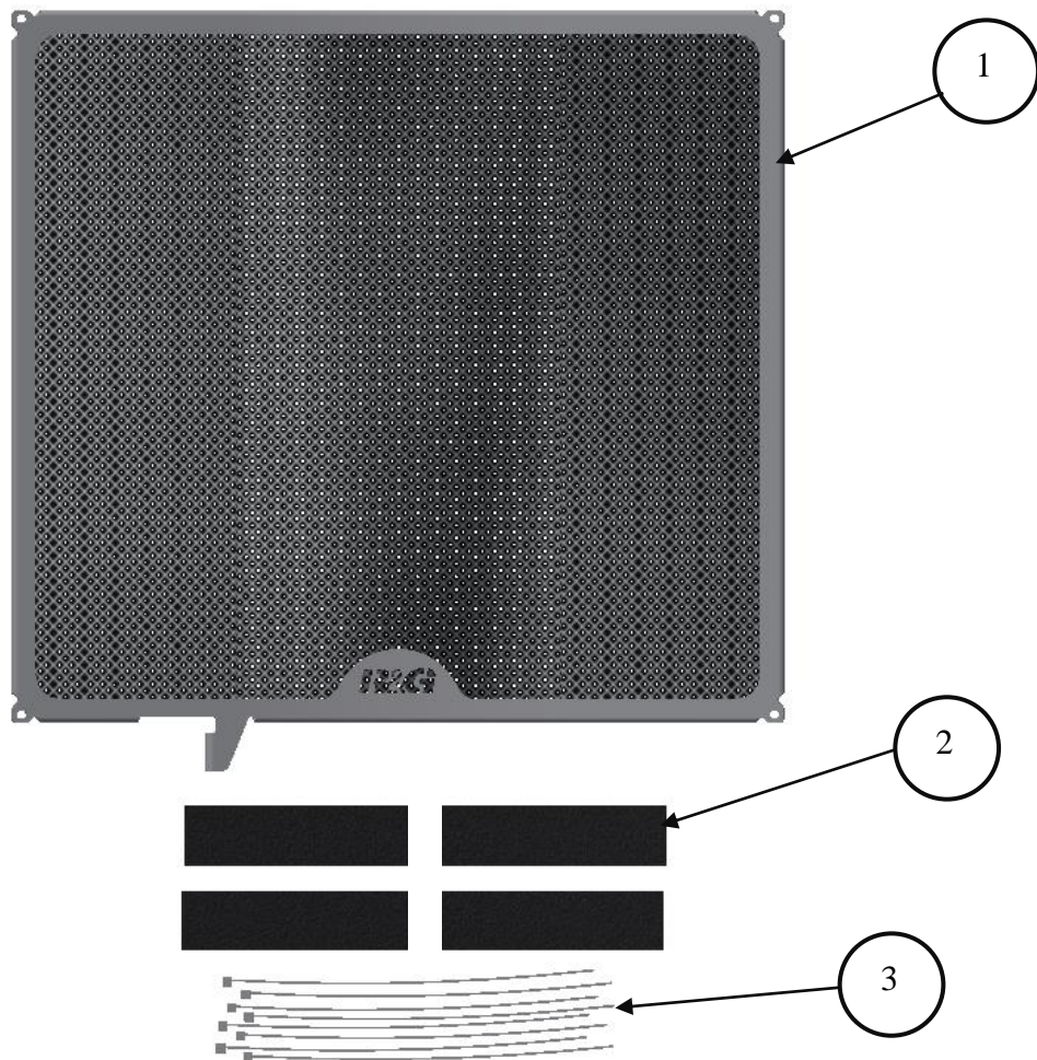
COMPONENT DIAGRAM
